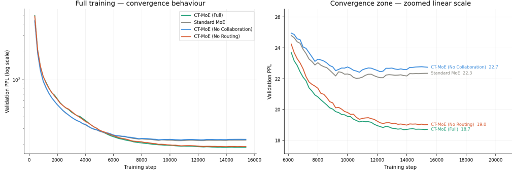
Figure 4: Validation perplexity over training steps, all four variants. CT-MoE-Full and CT-MoE-NoRouting diverge from StandardMoE and CT-MoE-NoCollab from approximately epoch 3 onward, coinciding with the first visible increase in S_{\max} above the uniform baseline.
